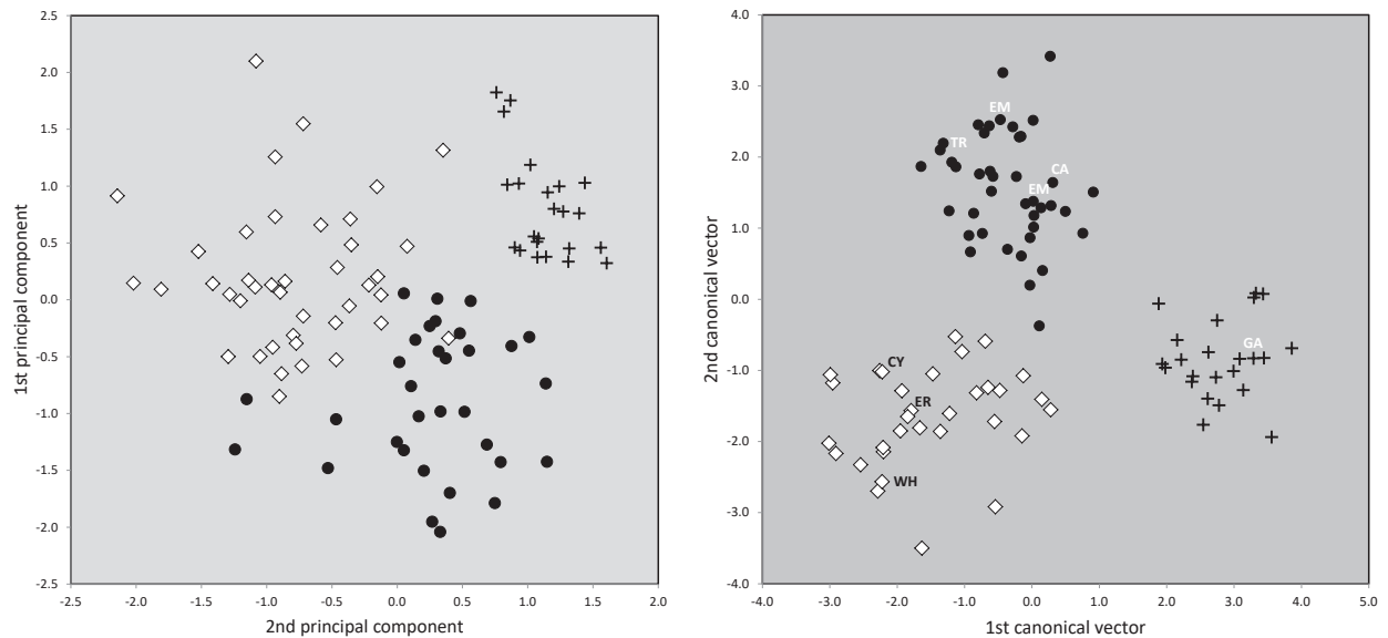
Figure 32 (left). Sample means of principal component analysis considering 12 characters measured in workers of Monomorium carbonarium (black dots), M. ergatogyna (white rhombs), and M. gallicum n.sp. (black crosses).
